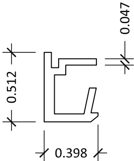
5 GLAZING BEAD
