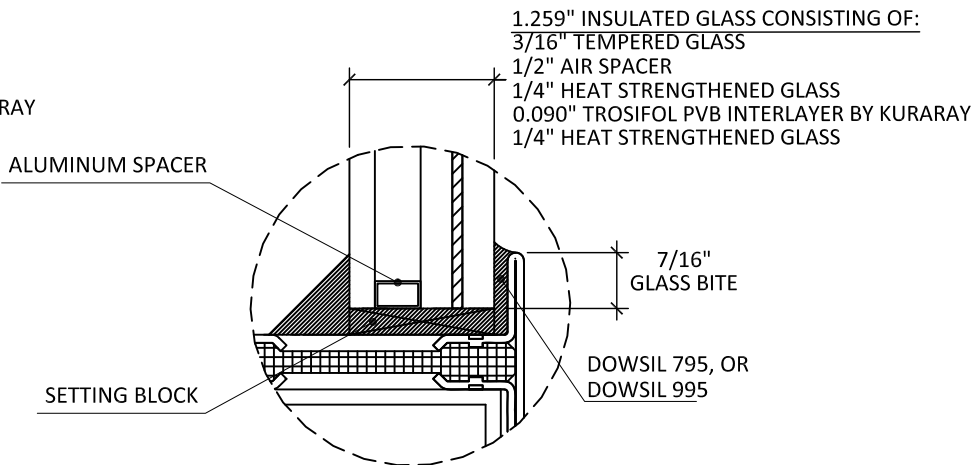
GLAZING DETAIL 3 GLASS TYPE G3
