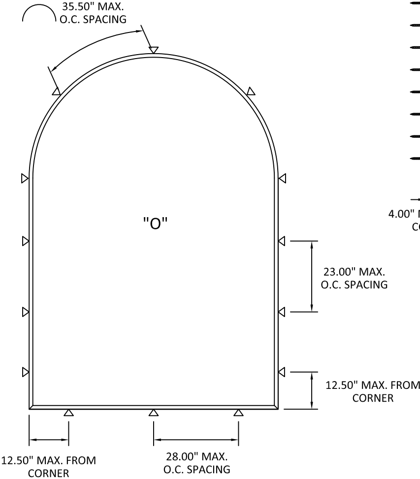
TYPICAL ANCHOR LAYOUT THROUGH BRACKET
