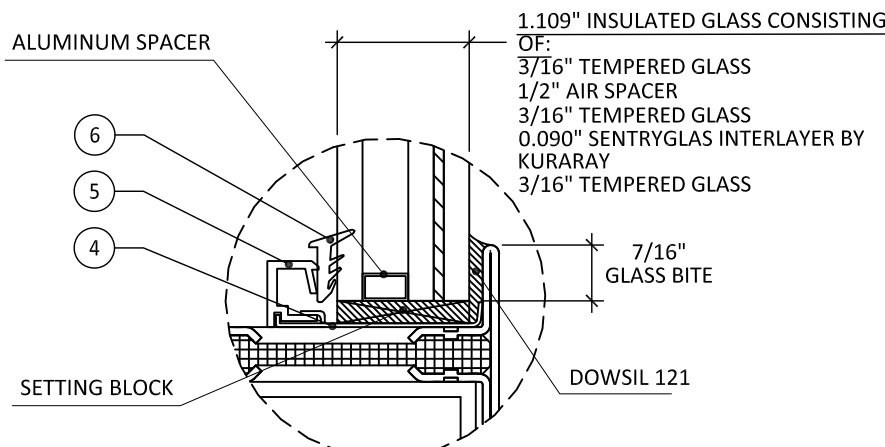
GLAZING DETAIL 1 GLASS TYPE G1
