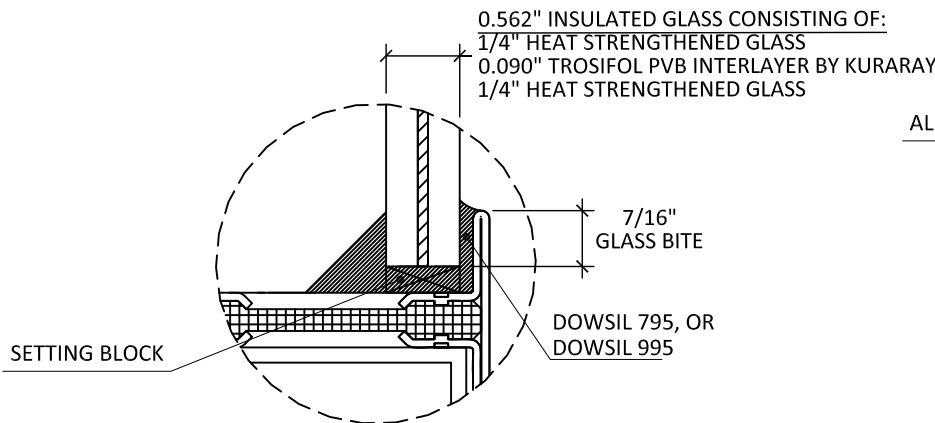
GLAZING DETAIL 2 GLASS TYPE G2
